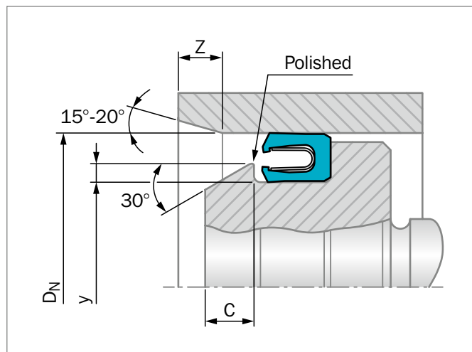
Figure 100: Installation in a half-open groove
