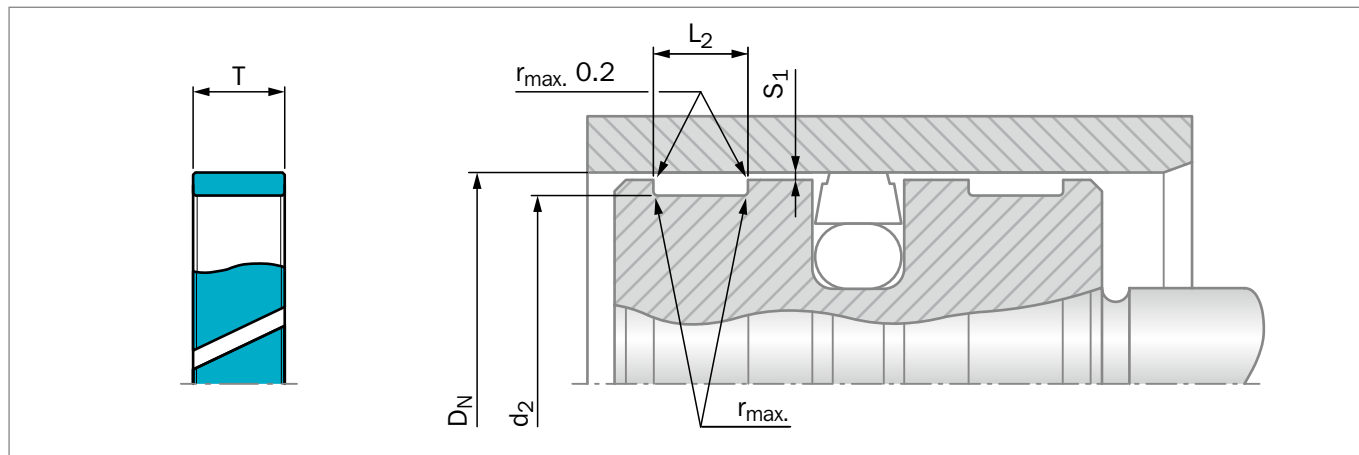
Figure 207: Piston guide
