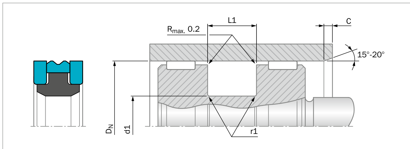
Figure 147: Installation Drawing
