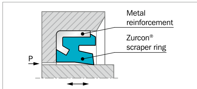
Figure 198: Scraper SWP
