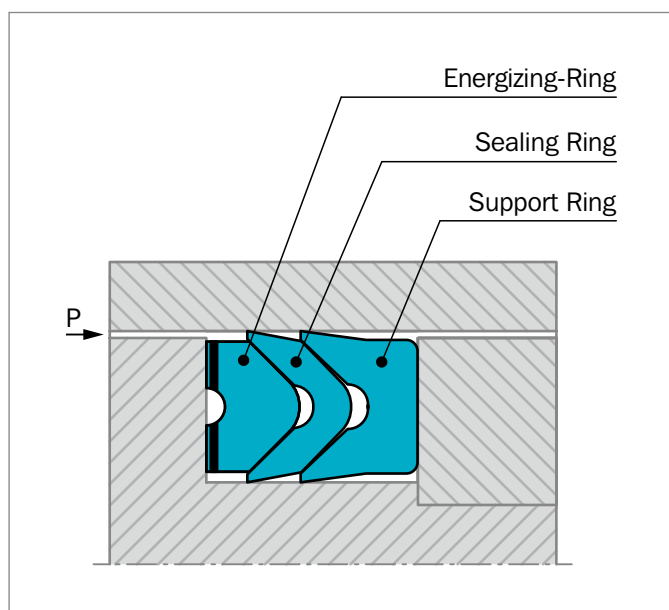
Figure 156: Veepac CH/G1
