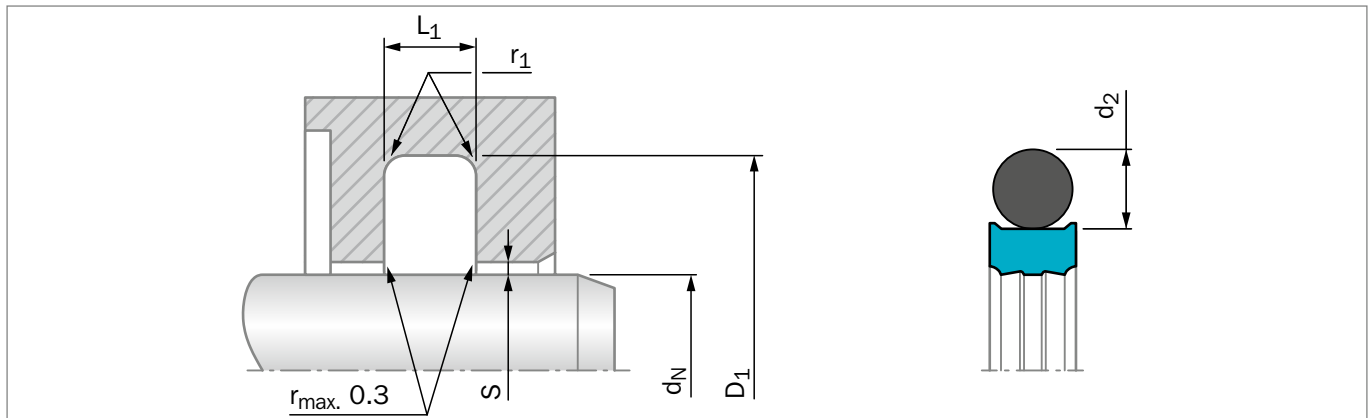
Figure 85: Installation Drawing
