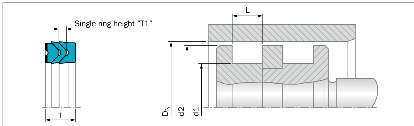
Figure 157: Installation Drawing
