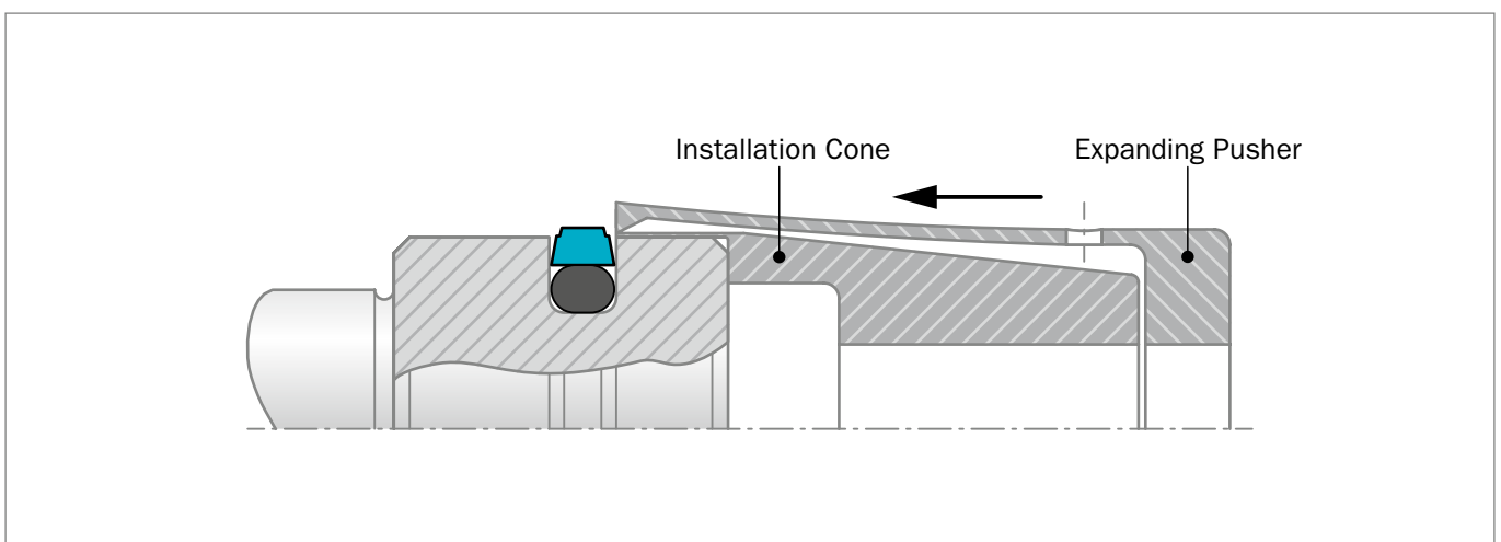
Figure 96: Sealing element after snapping into the groove
