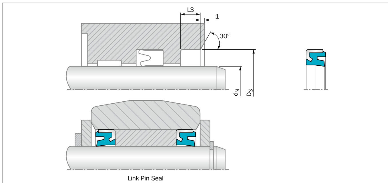
Figure 199: Installation Drawing
