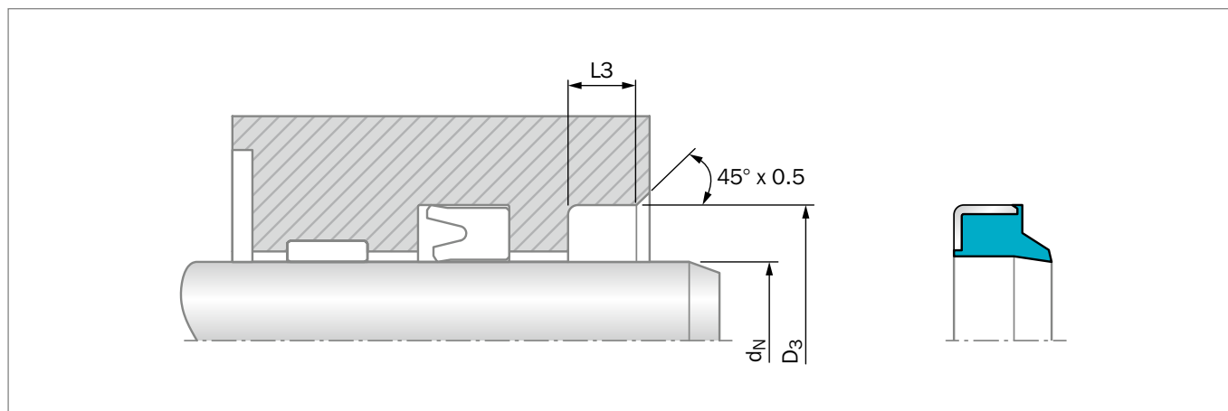
Figure 197: Installation Drawing
