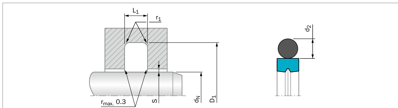
Figure 78: Installation Drawing
