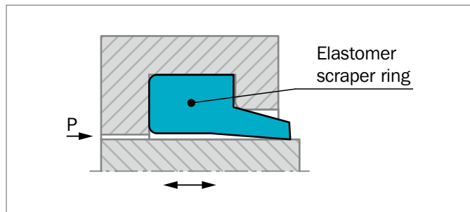
Figure 190: Scraper WRM
