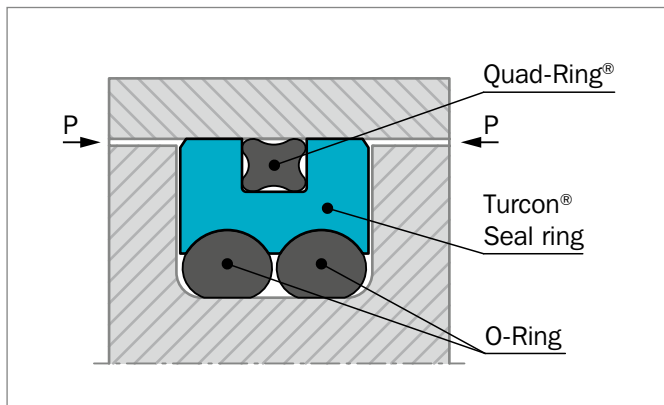
Figure 116: Turcon® AQ-Seal® 5
