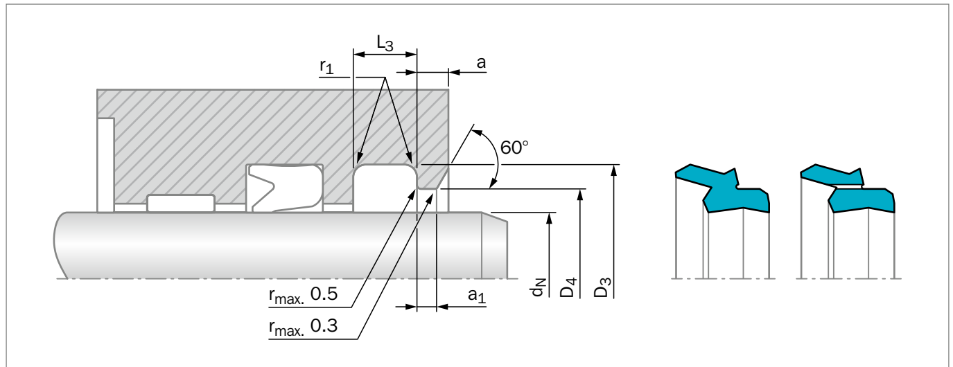
Figure 189: Installation Drawing
