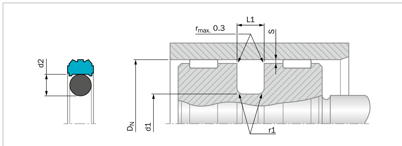
Figure 142: Installation Drawing
