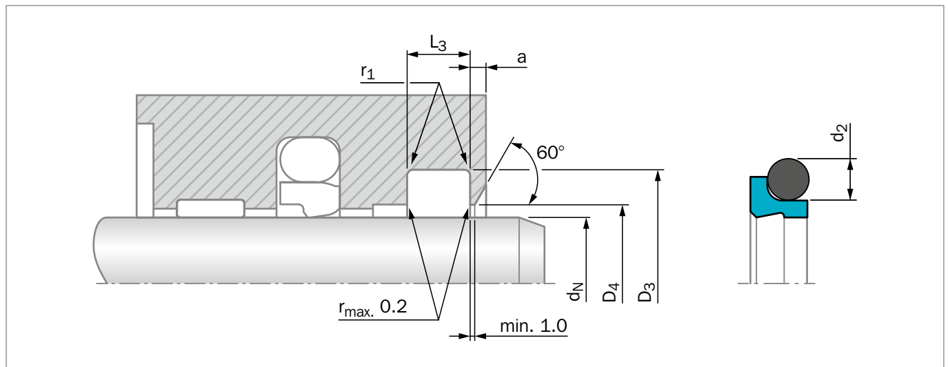
Figure 161: Installation Drawing
