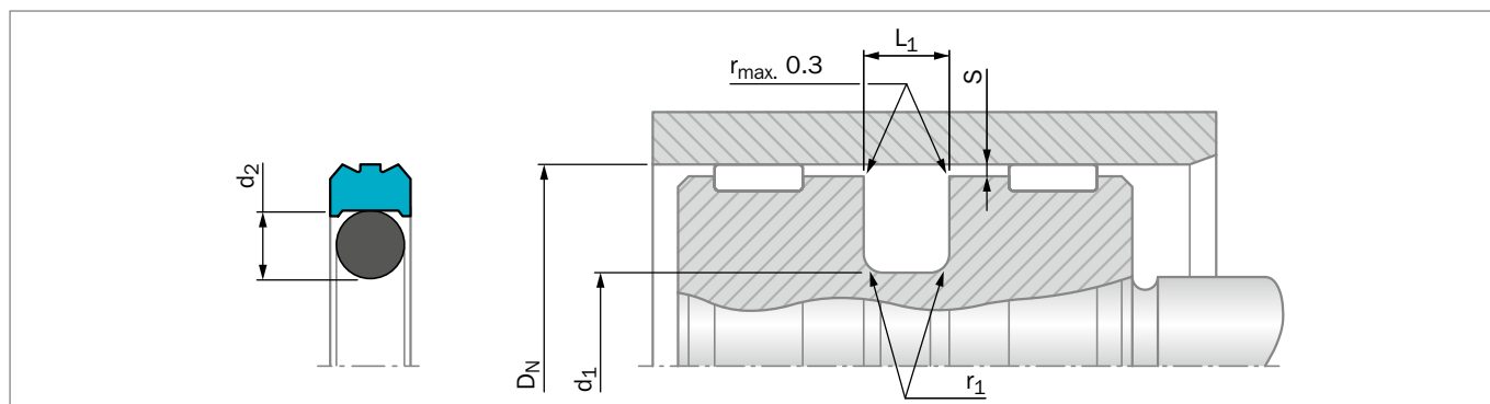
Figure 145: Installation Drawing
