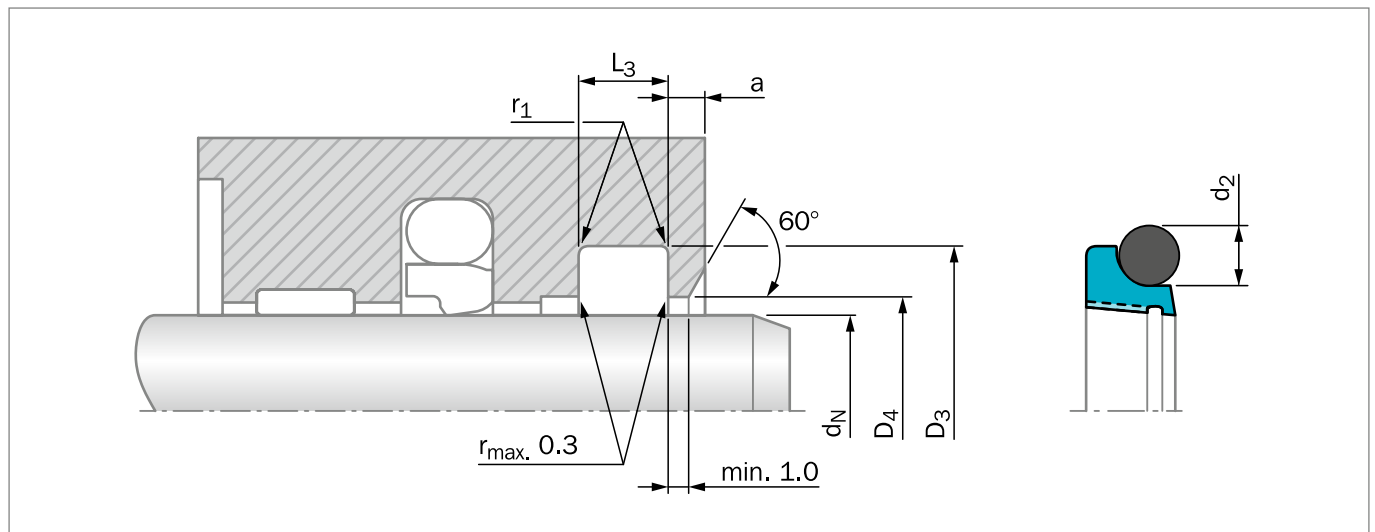
Figure 182: Installation Drawing
