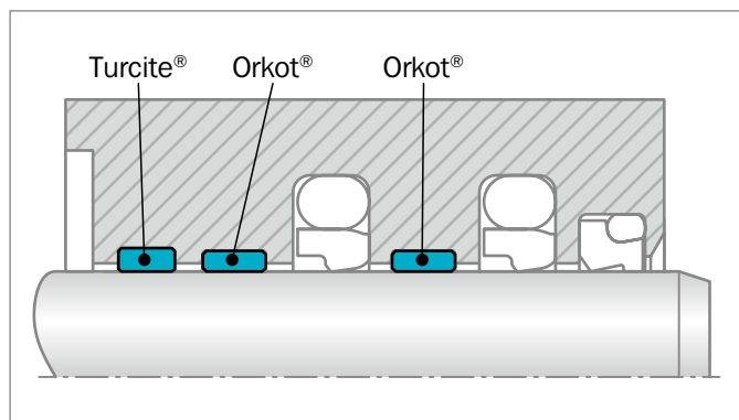
Figure 209: Rod guide for high loads (See also Figure 222 page 606)
