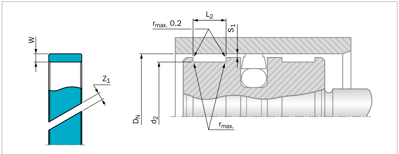
Figure 215: Installation Drawing
