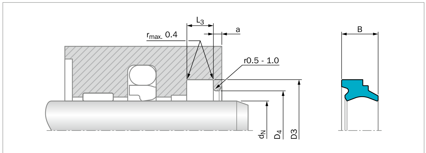
Figure 184: Installation Drawing
