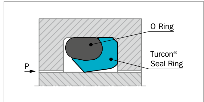
Figure 66: Turcon® VL Seal® mounted in O-Ring groove
