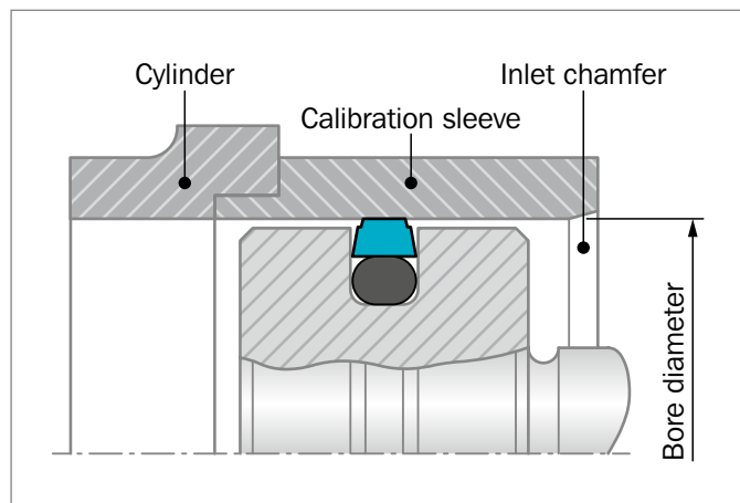
Figure 97: Sizing the sealing element with calibration sleeve
