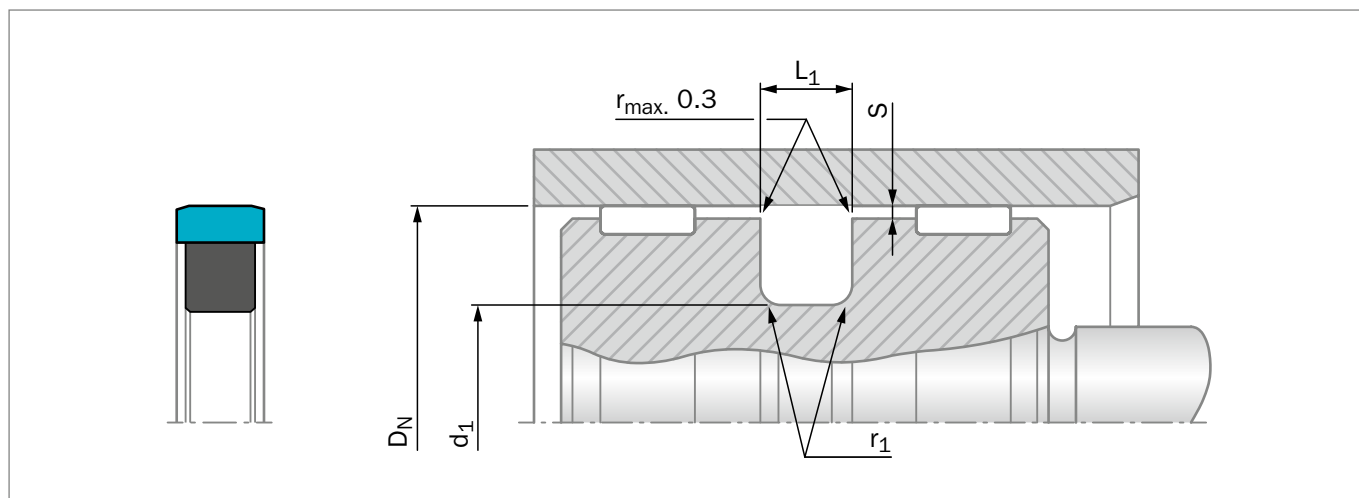
Figure 115: Installation Drawing
