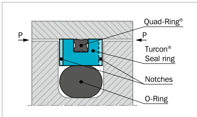
Figure 118: Turcon® AQ-Seal®
