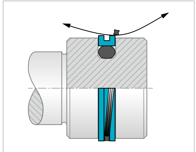
Figure 101: Installation of Quad-Ring® in AQ-Seal® for piston.
