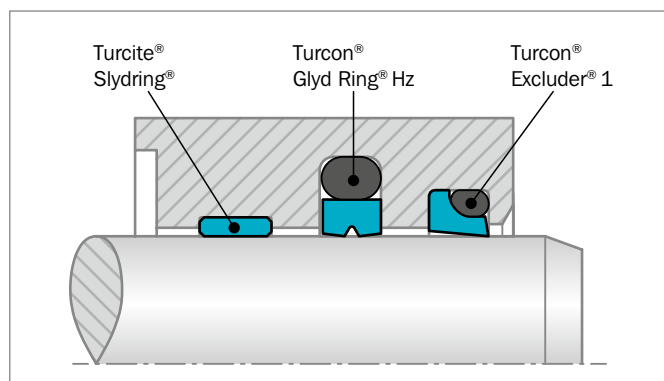
Figure 77: Glyd Ring® Hz with Turcon® Excluder® 1 and Turcite® Slydring®
