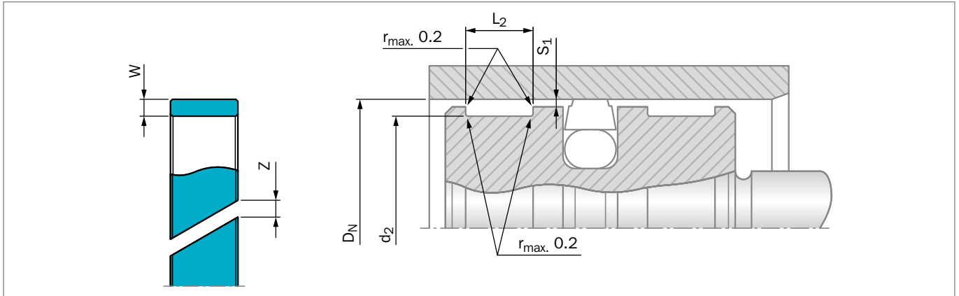
Figure 213: Installation Drawing
