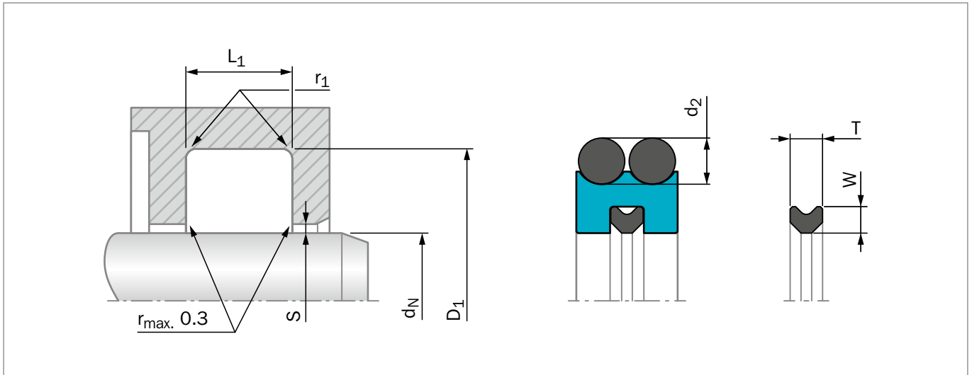
Figure 82: Installation Drawing
