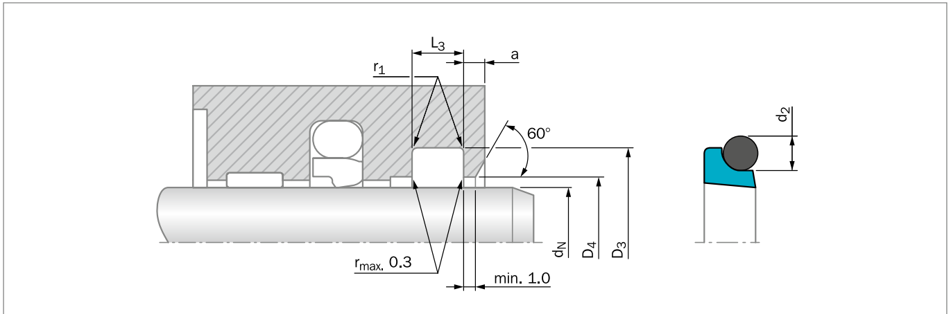
Figure 180: Installation Drawing
