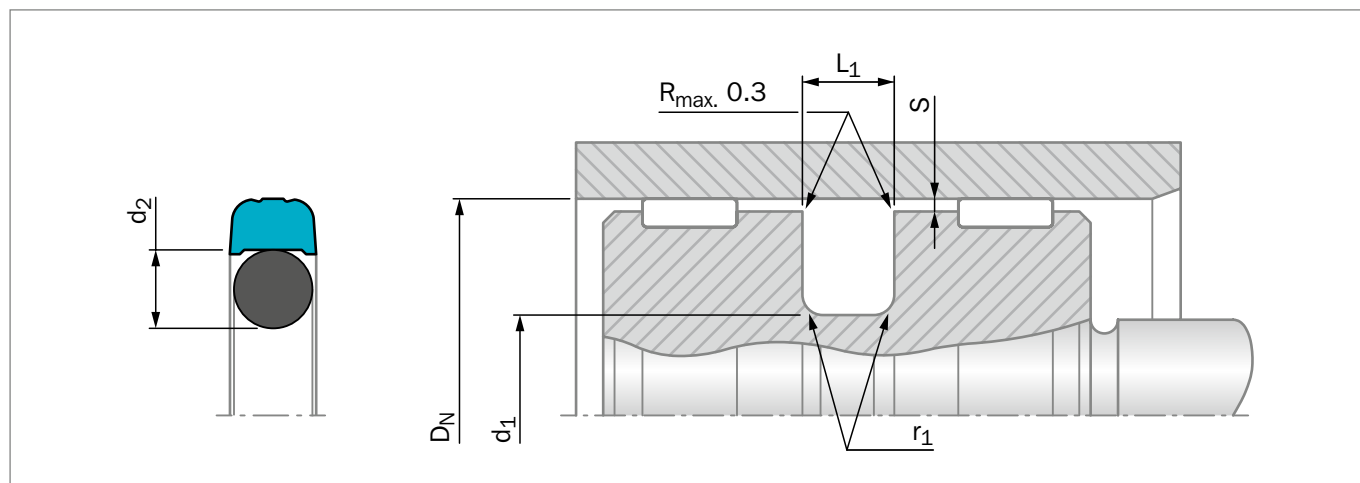
Figure 112: Installation Drawing
