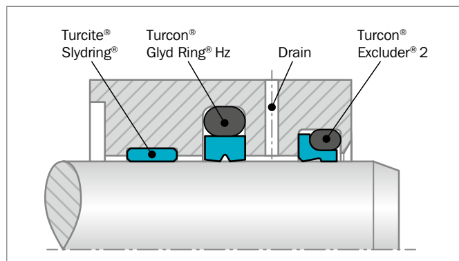
Figure 76: Glyd Ring® Hz with Turcon® Excluder® 2 and Turcite® Slydring®
