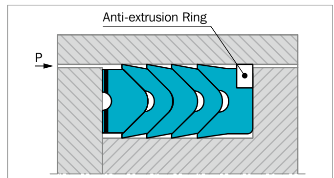
Figure 154: Veepac design with anti-extrusion ring
