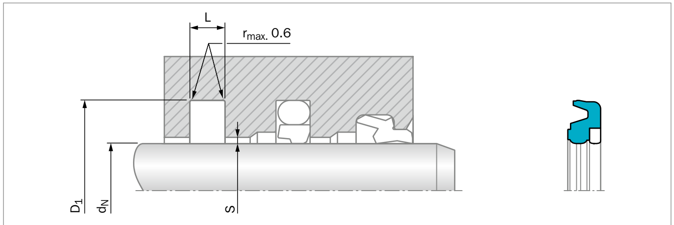
Figure 60: Installation Drawing
