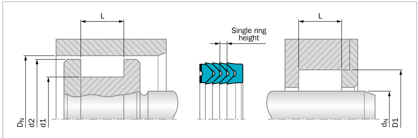
Figure 155: Installation Drawing
