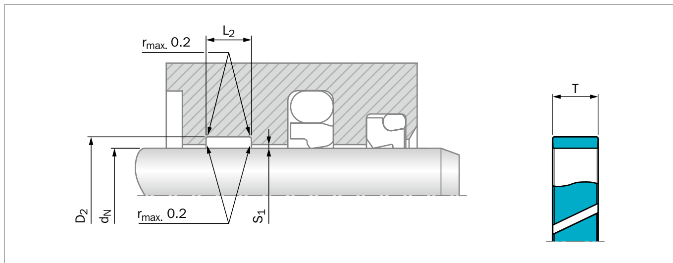
Figure 208: Rod guide
